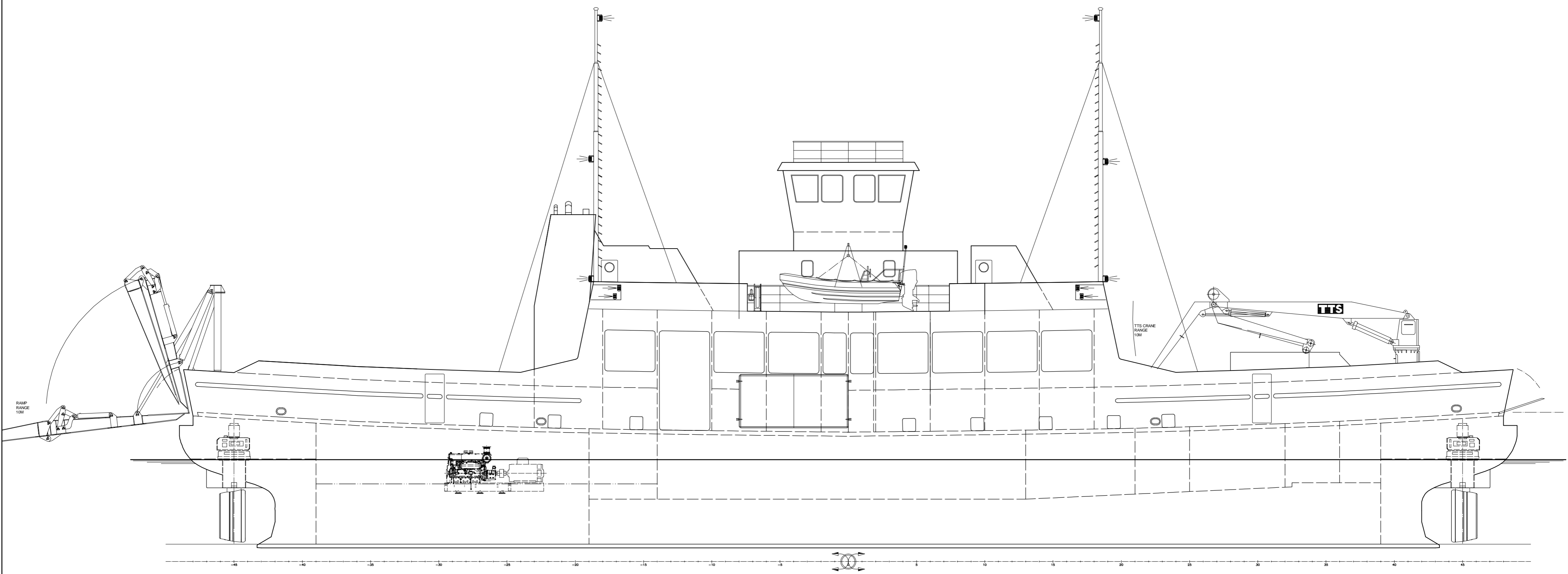
PROFILE STARBOARD
