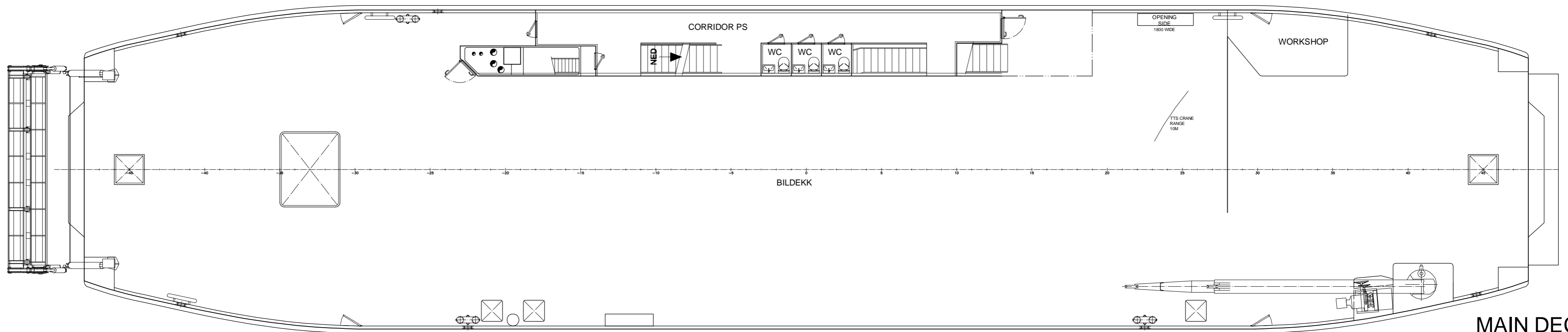
MAIN DECK
