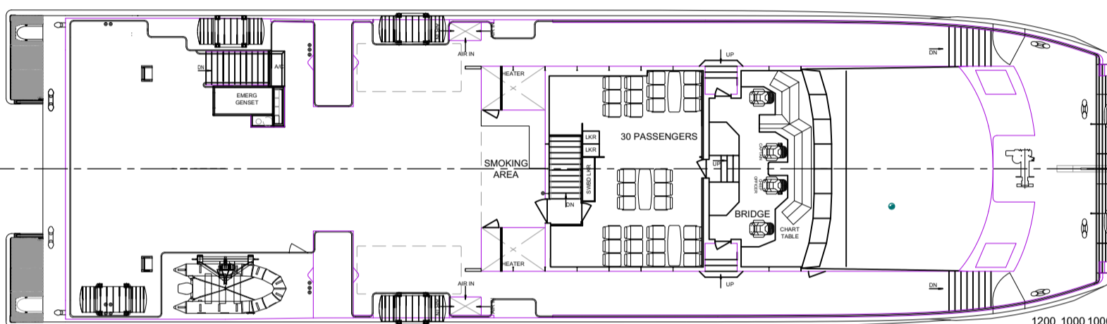
UPPER DECK
