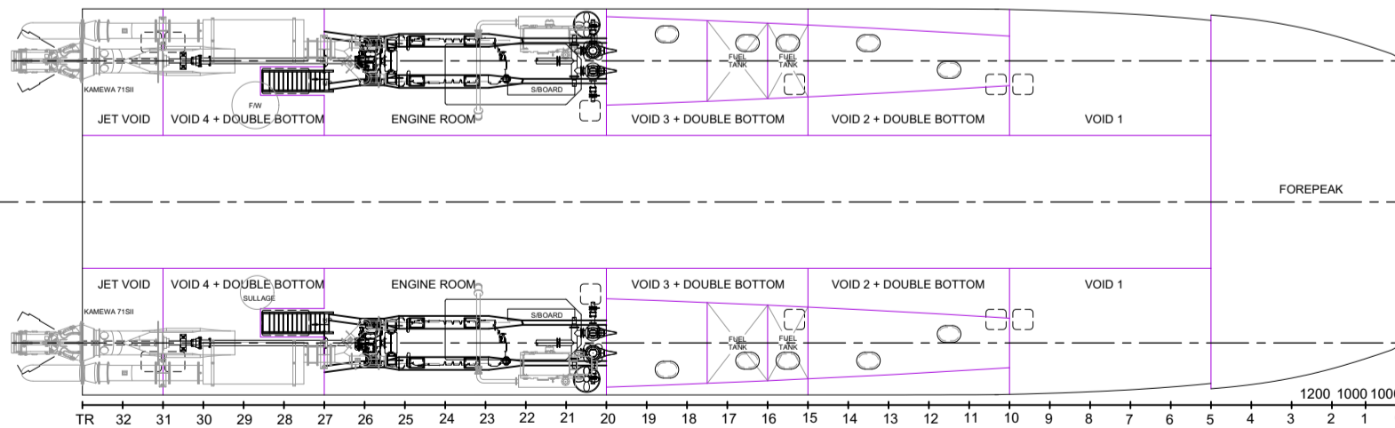
HULLS
