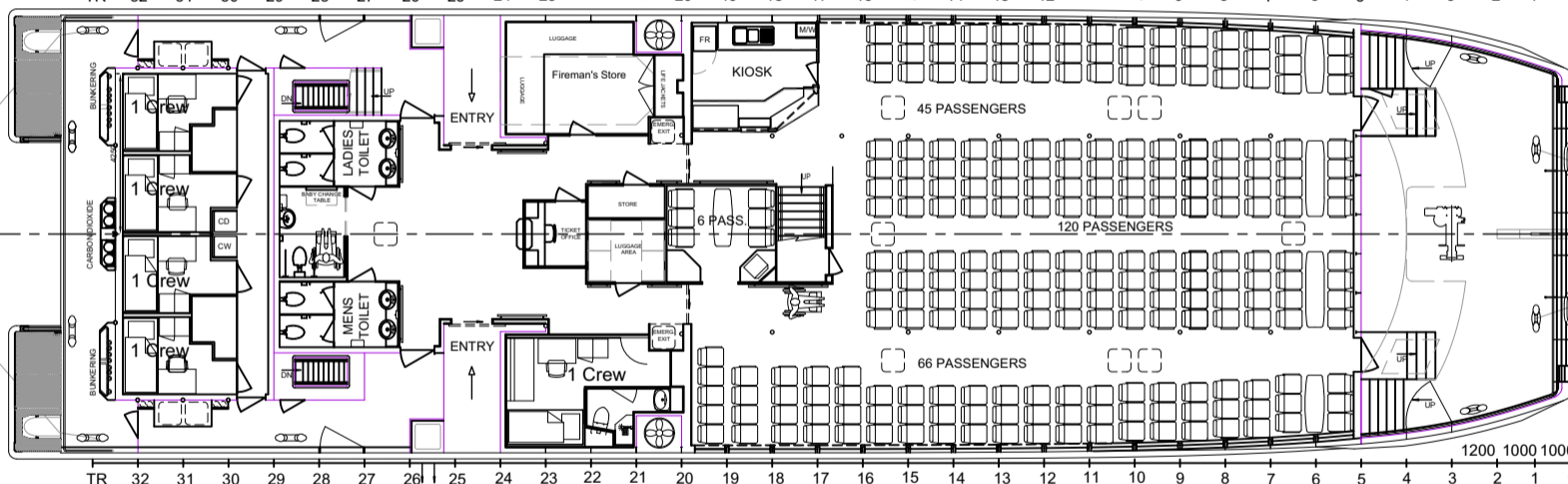
MAIN DECK
