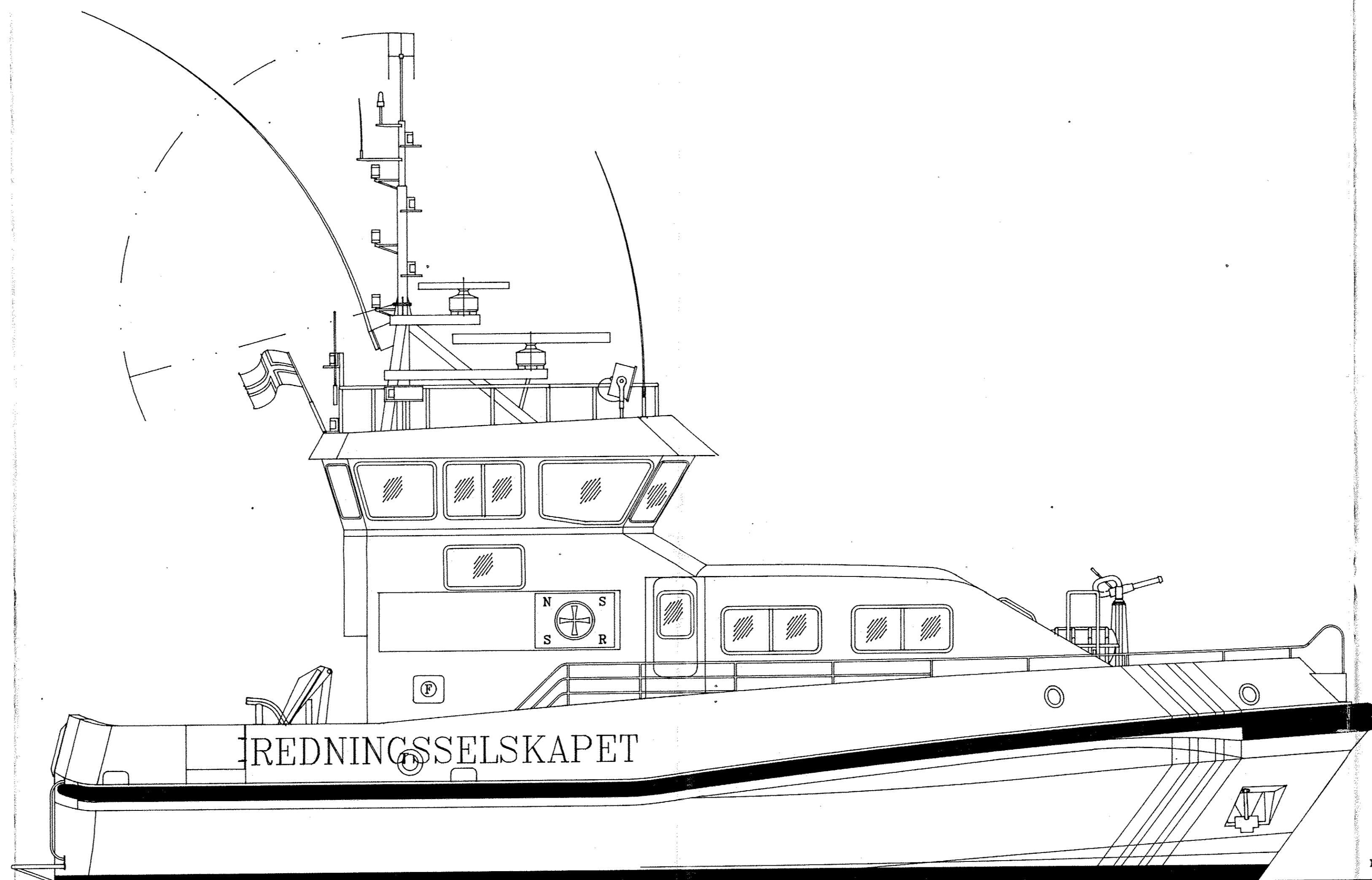
Outboard Profile
