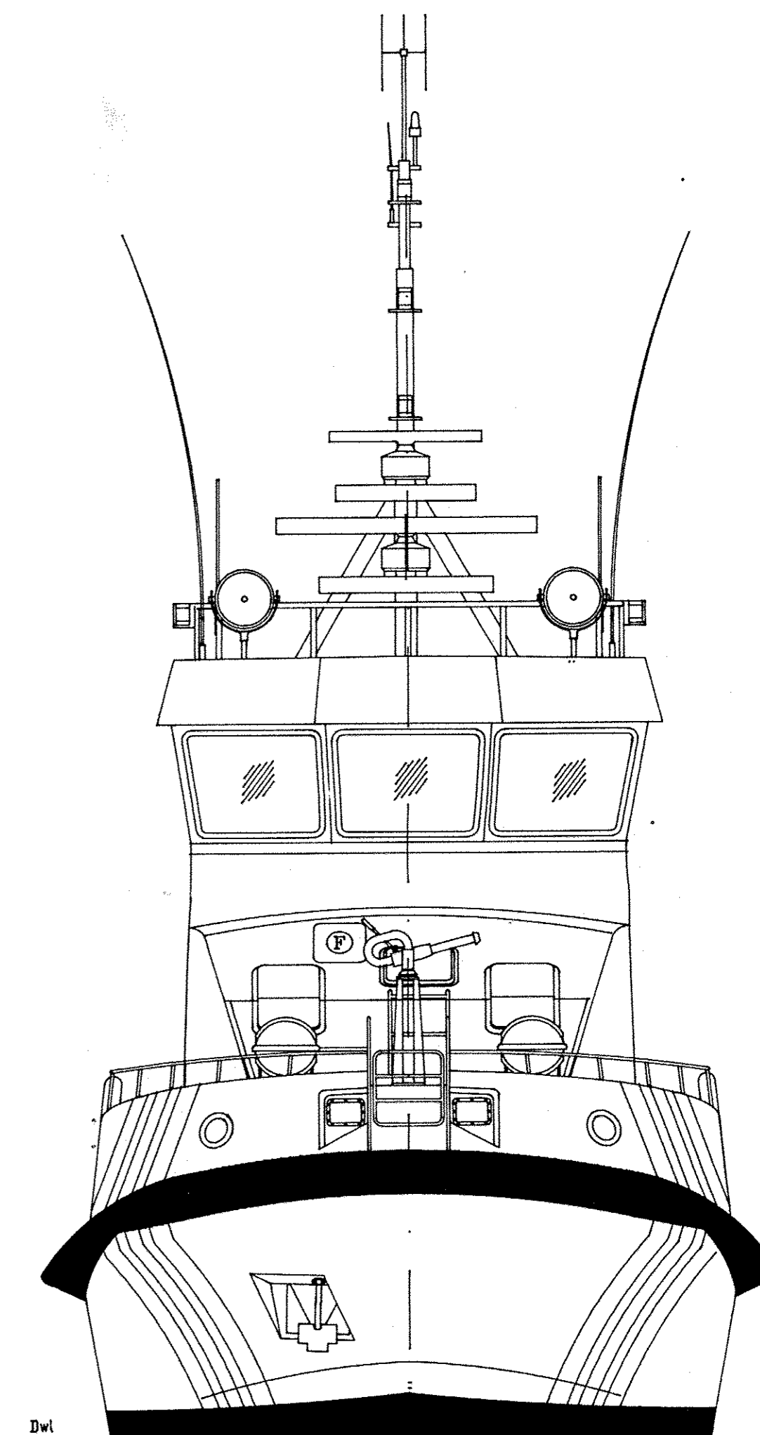
Bow View
