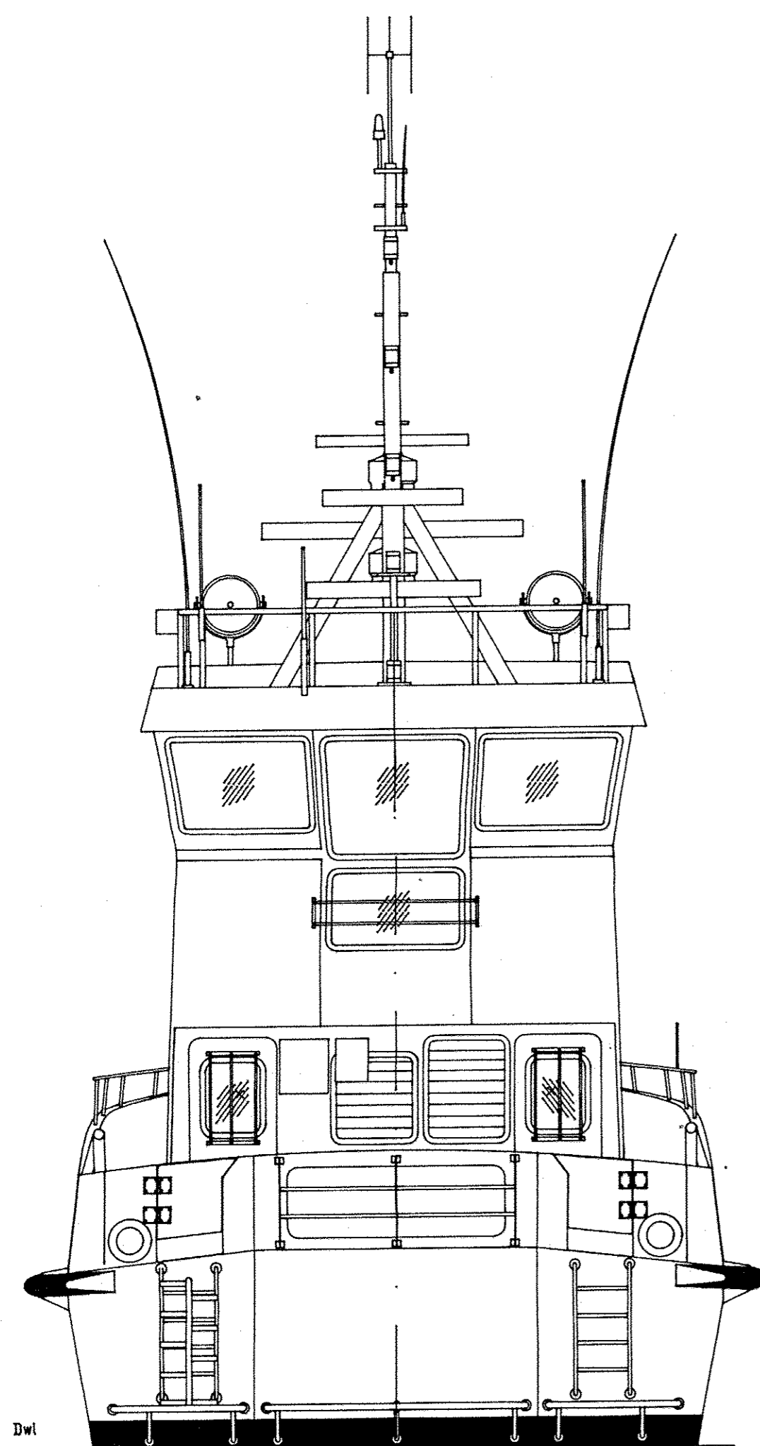
Stern View
